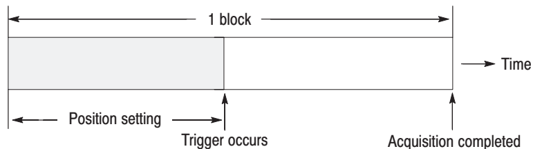
Figure 3-70: Trigger position
