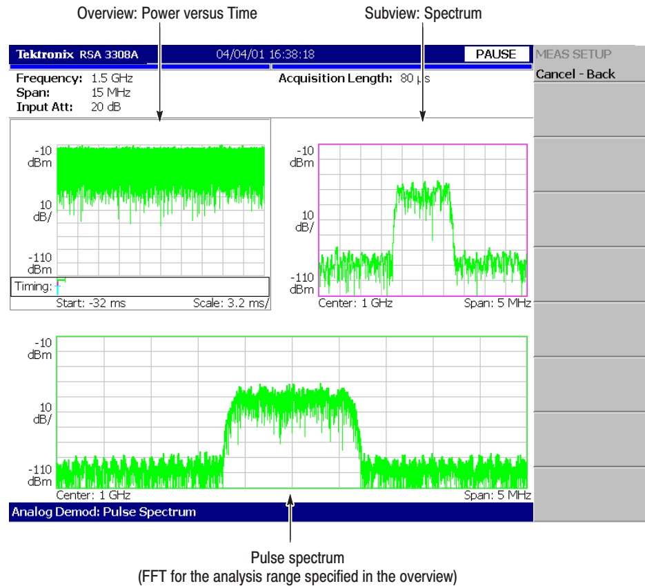
Figure 3–37: Pulse spectrum measurement
