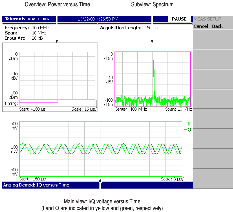
Figure 3–36: IQ versus time measurement
