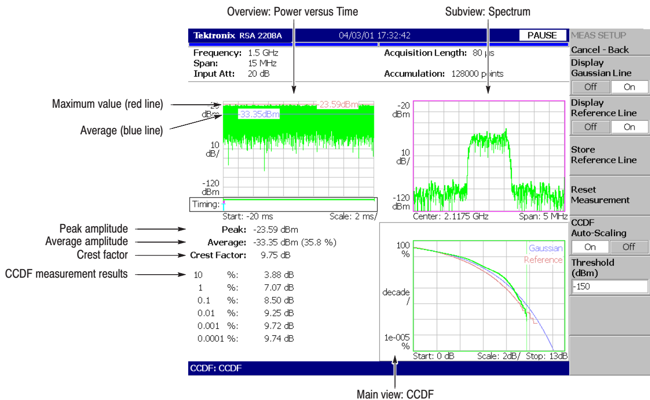
Figure 3–44: CCDF multi-view
