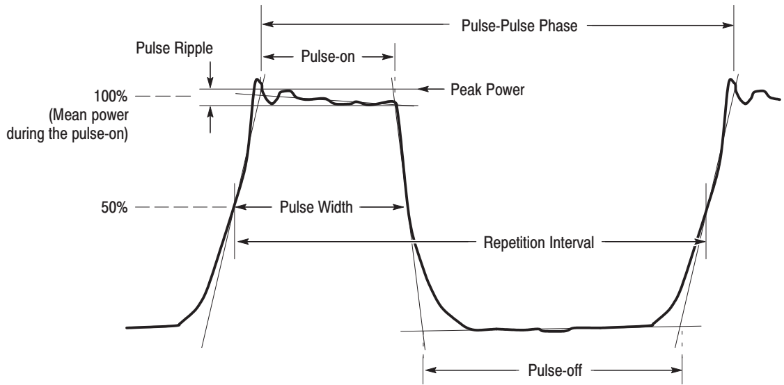
Figure 3-45: Definition of pulse characteristics
