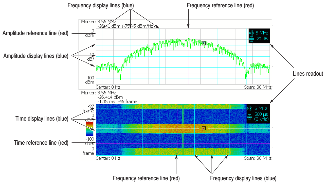
Figure 3–97: Multi display lines (Real Time S/A mode)
