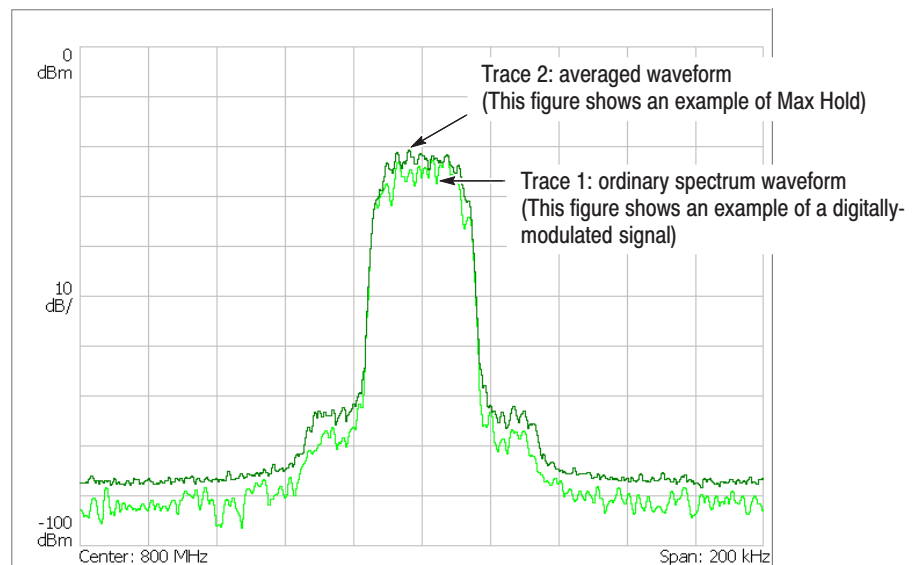
Figure 3–85: Compared display
