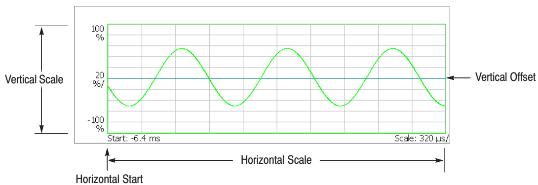
Figure 3-91: Setting the scale in time domain view
