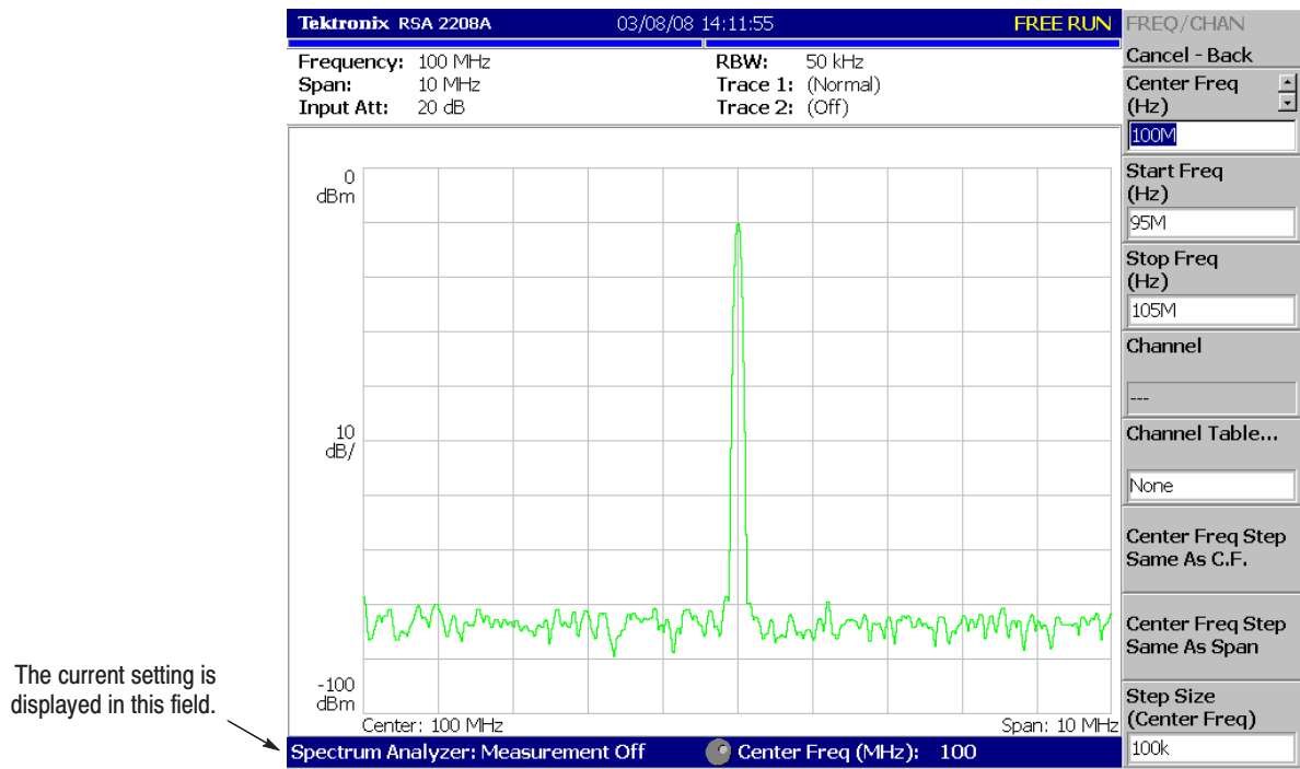
Figure 2–33: Center frequency of 100 MHz, span of 10 MHz
