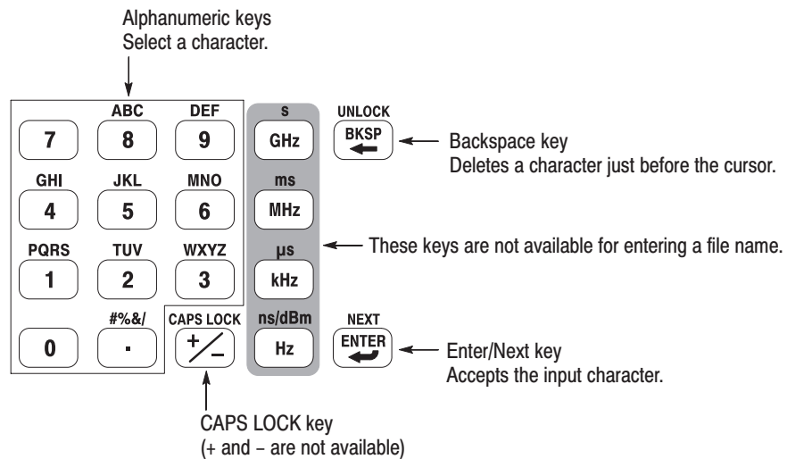
Figure 3–118: Alphanumeric keypad
