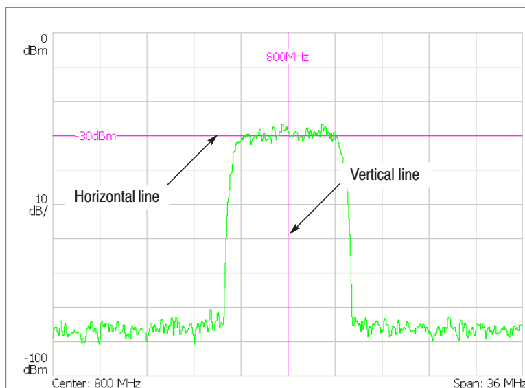
Figure 3–93: Display line
