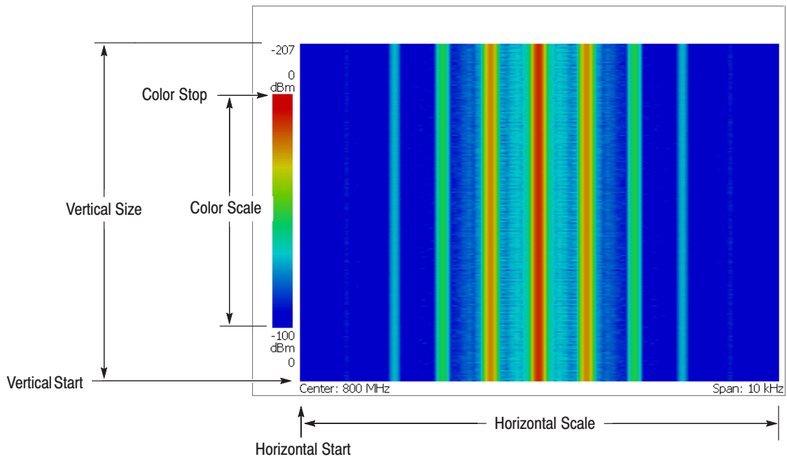
Figure 3-90: Scale and format settings in spectrogram view
