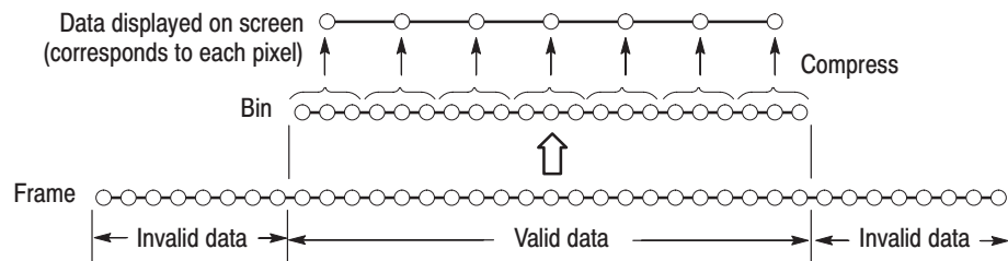
Figure 3-86: Relationships between frame, bin, and pixel
