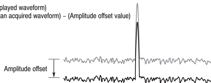
Figure 3–60: Amplitude offset
