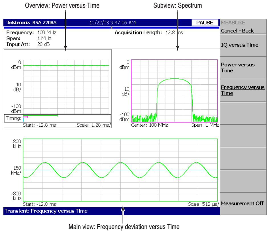
Figure 3–41: Frequency measurement
