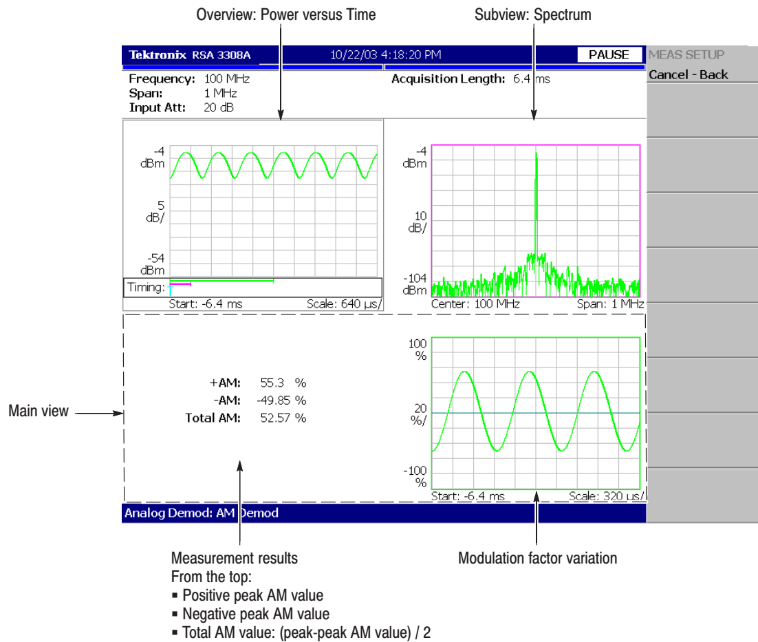
Figure 3–33: AM demod measurement
