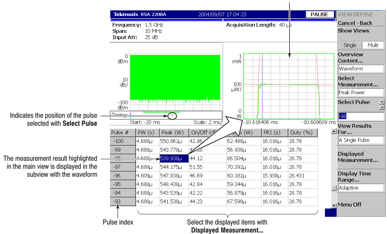
Figure 3–48: Setting the View Define menu
