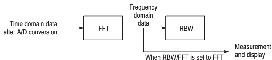
Figure 3–78: Process flow when RBW/FFT = FFT
