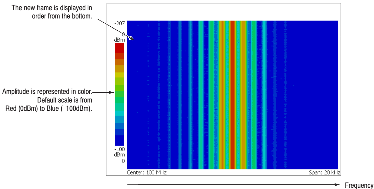
Figure 2–46: Spectrogram view
