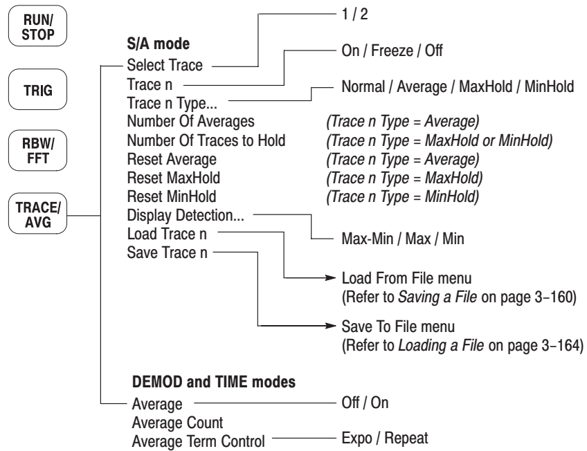
Figure 3-83: RBW/FFT menu structure
