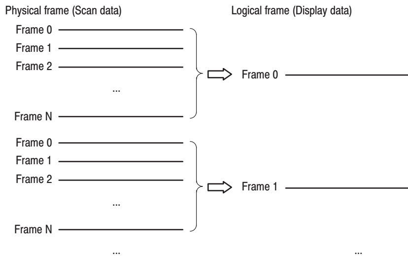
Figure 3–53: Vector mode and scalar mode
