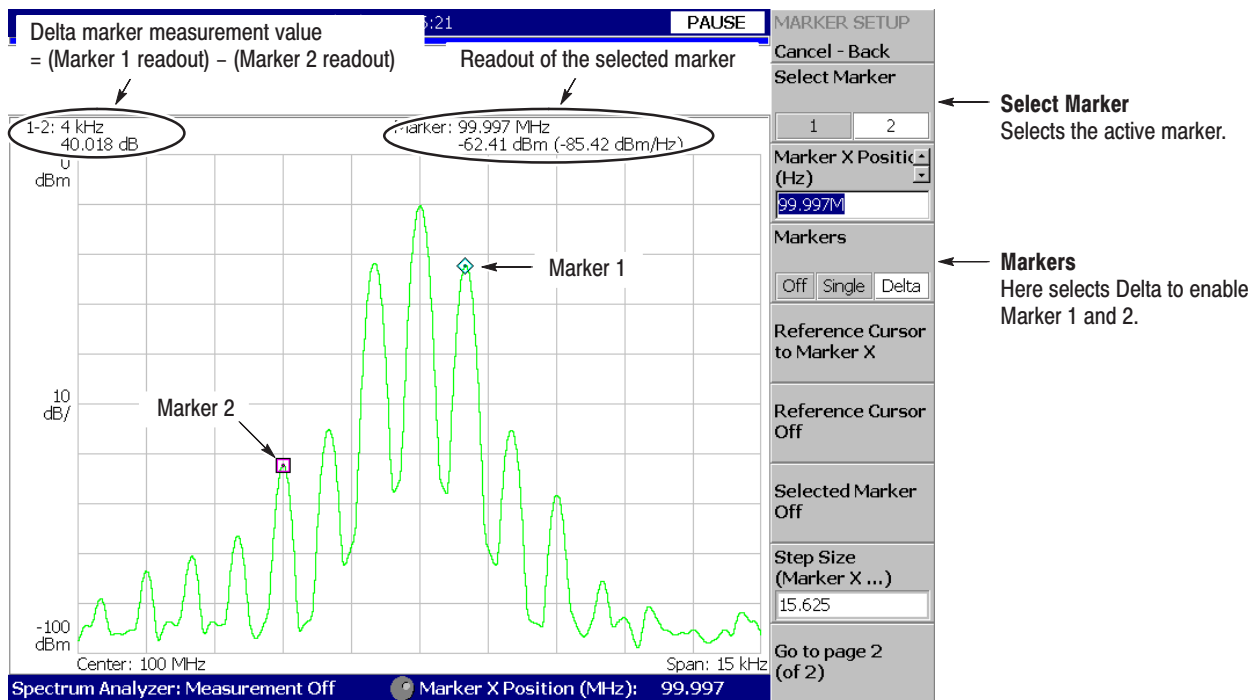
Figure 3–102: Using the delta marker to take measurements
