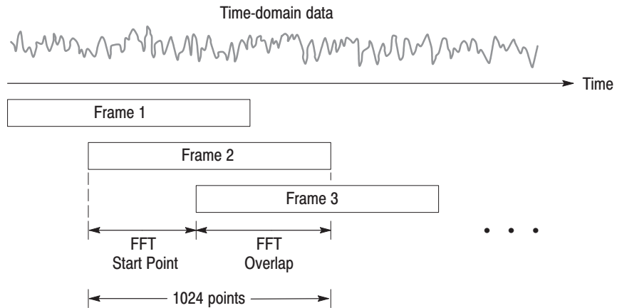
Figure 3–79: FFT overlap
