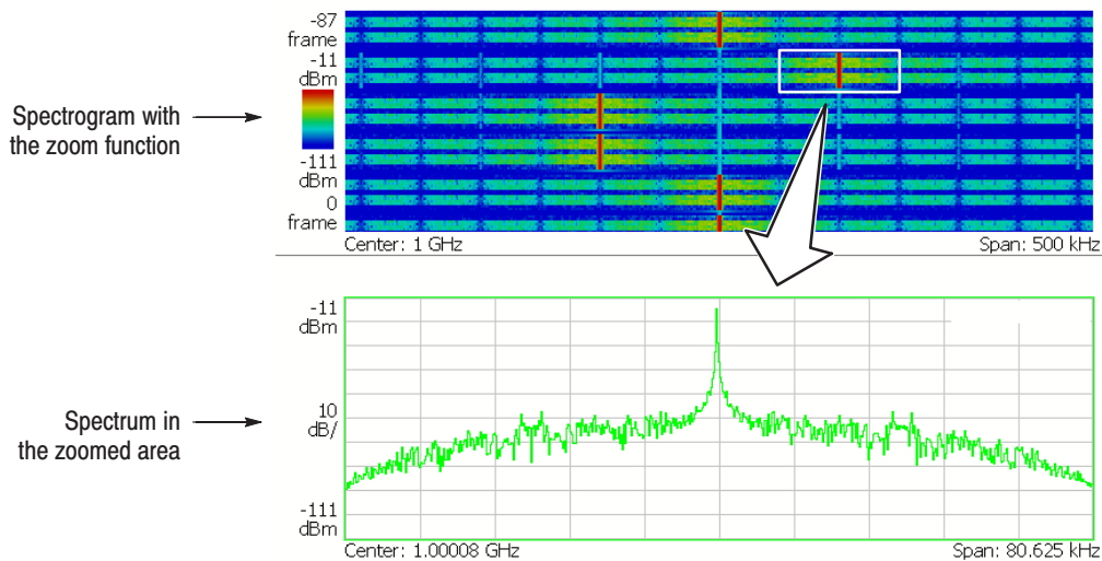
Figure 3–22: Zoom function
