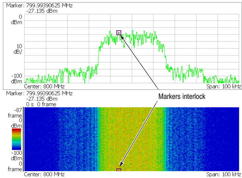
Figure 3–105: Interlocked markers
