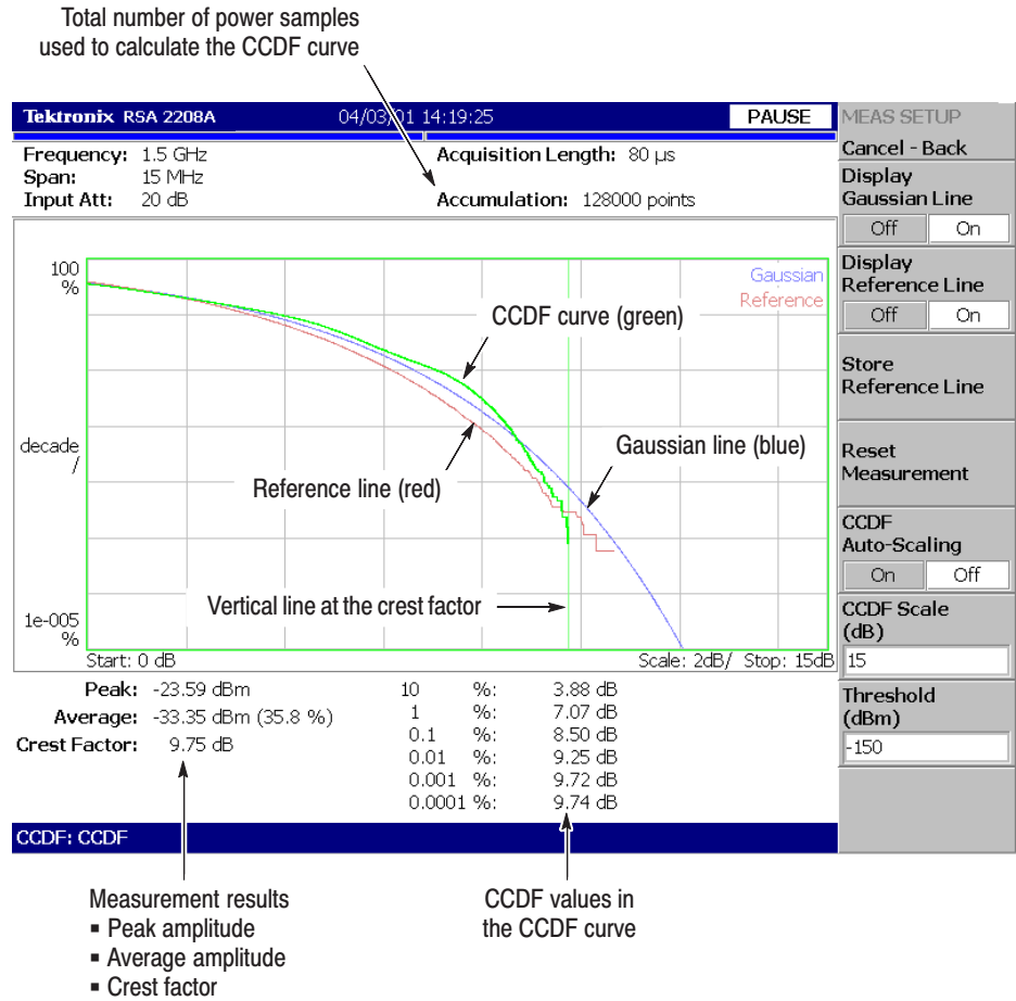
Figure 3–43: CCDF single view
