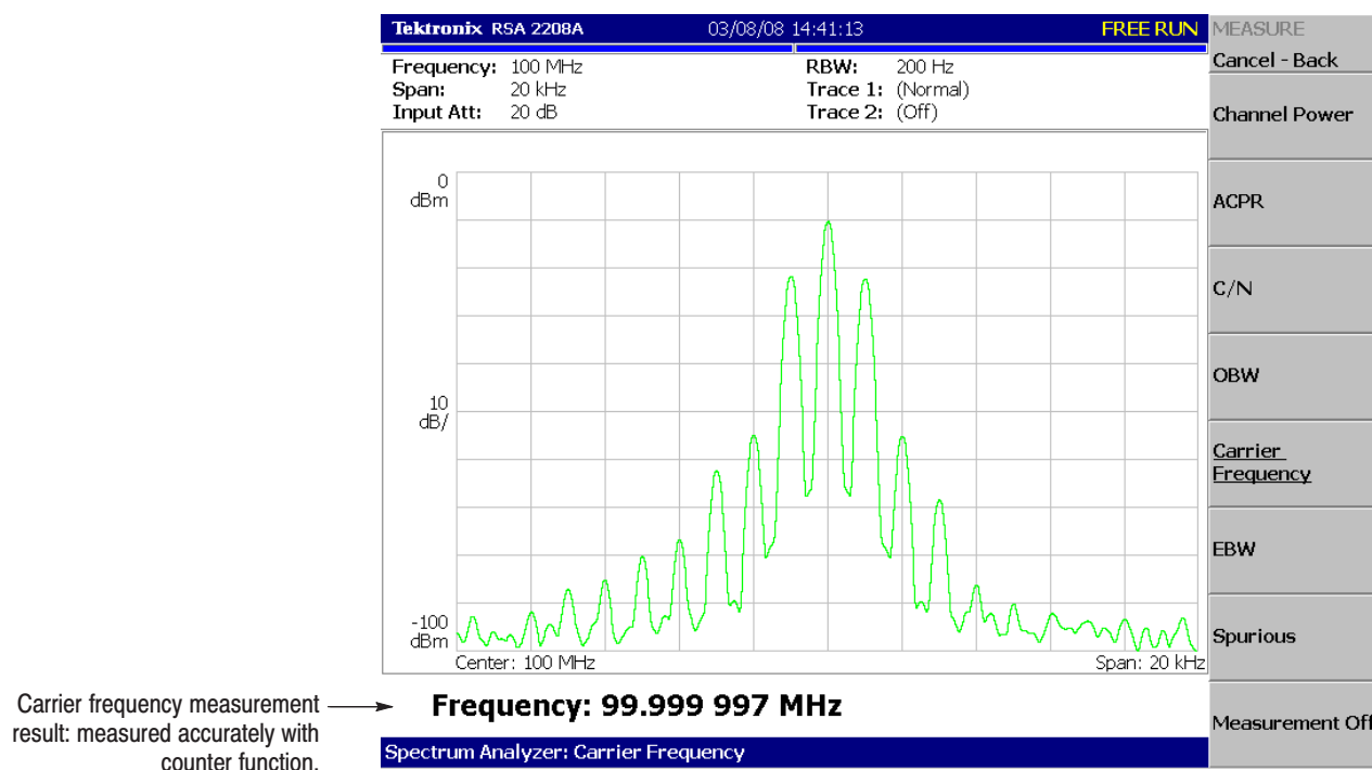
Figure 2–49: Carrier frequency measurement
