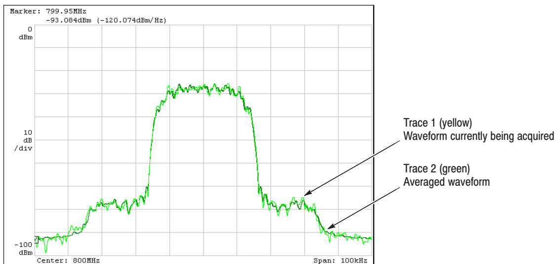
Figure 3–82: Comparison display of Trace 1 and 2
